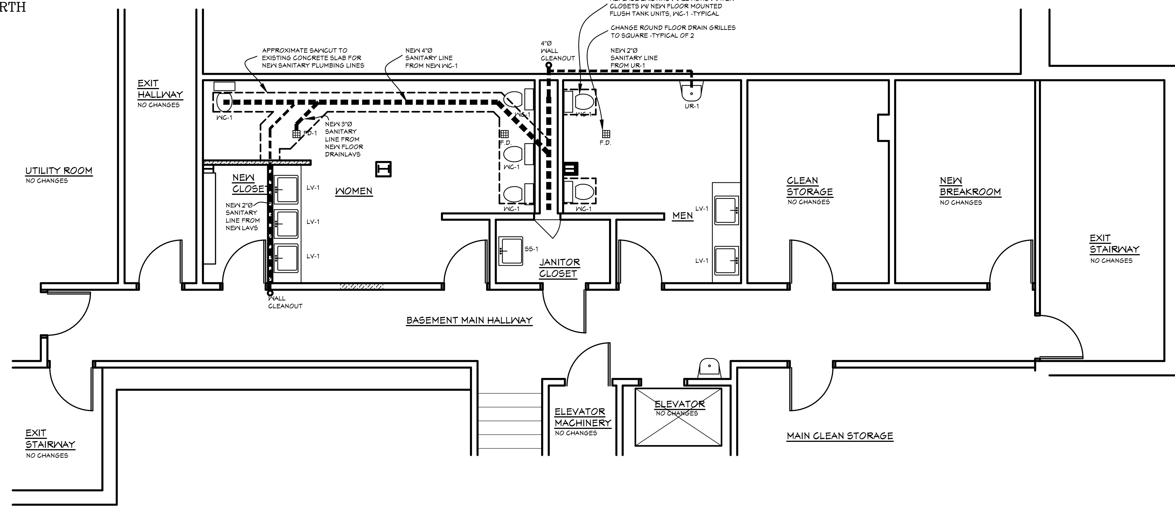
PROPOSED PARTIAL BASEMENT PLUMBING PLAN
